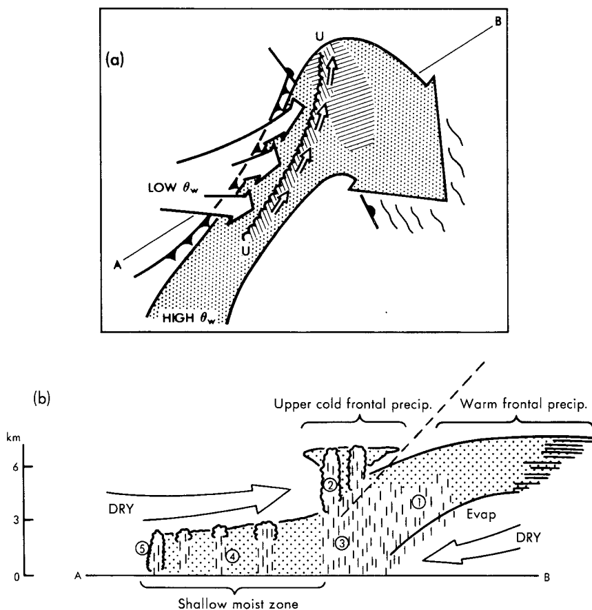
FIG. 5. Schematic portrayal of the same situation as in Fig. 4, i.e., with the warm conveyor belt undergoing forward-sloping ascent but drawing attention to the split-front characteristic and the overall precipitation distribution: (a) plan view; (b) vertical section along AB in (a). In (a) UU represents the upper cold front. The hatched shading along UU and ahead of the warm front represents precipitation associated with the upper cold front and warm front, respectively. Numbers in (b) represent precipitation type as follows: 1) warm frontal precipitation, 2) convective precipitation-generating cells associated with the upper cold front, 3) precipitation from the upper cold frontal convection descending through an area of warm advection, 4) shallow moist zone between the upper and surface cold fronts characterized by warm advection and scattered outbreaks of mainly light rain and drizzle, and 5) shallow precipitation at the surface cold front itself (after Browning and Monk, 1982).
