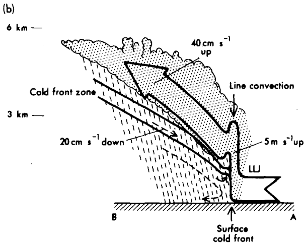
FIG. 3. Schematic portrayal of airflow at a classical ana cold front showing the warm conveyor belt (bold arrow) undergoing rearward-sloping ascent above the cold frontal zone with the cold air (dashed lines) descending beneath it: (a) plan view; (b) vertical section along AB in (a). Flows are shown relative to the moving frontal system. LLJ marks axis of low-level jet in (b).
